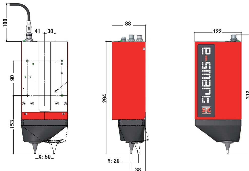
Marking window - 50 x 20 mm
